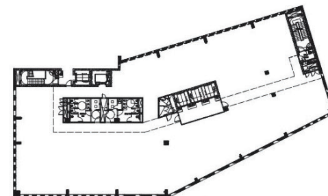
FLOOR LEVEL 5
